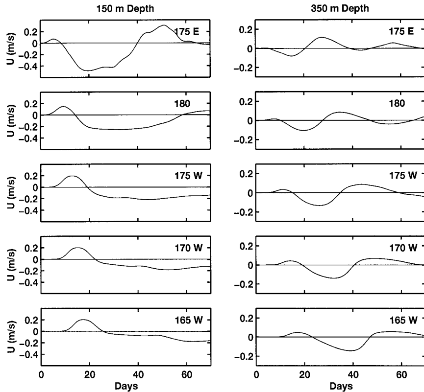
FIG. 5. Time series of the zonal velocity at 150- and 350-m depths at various longitudes for expt 1.
