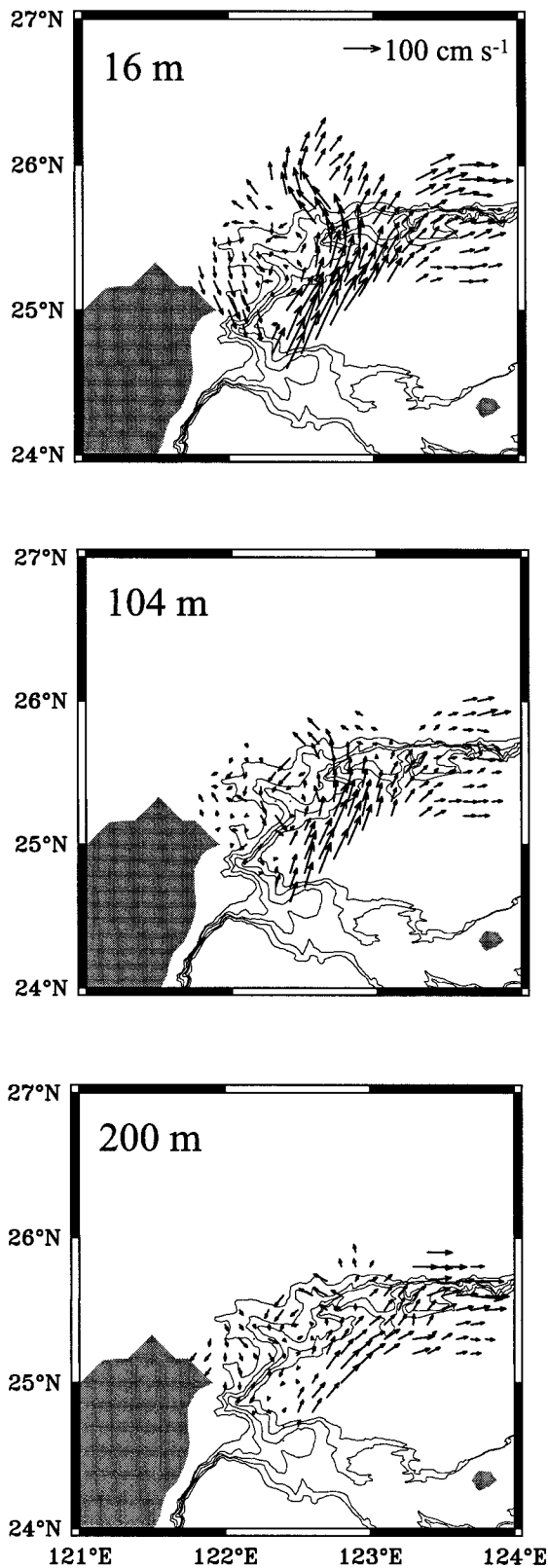
FIG. 2. Phase-averaged current vectors from SADC observations at depth (a) 16, (b) 104, and (c) 200 m. The bathymetry is shown with thin depth contours from 200 to 1000 m at intervals of 200 m.
