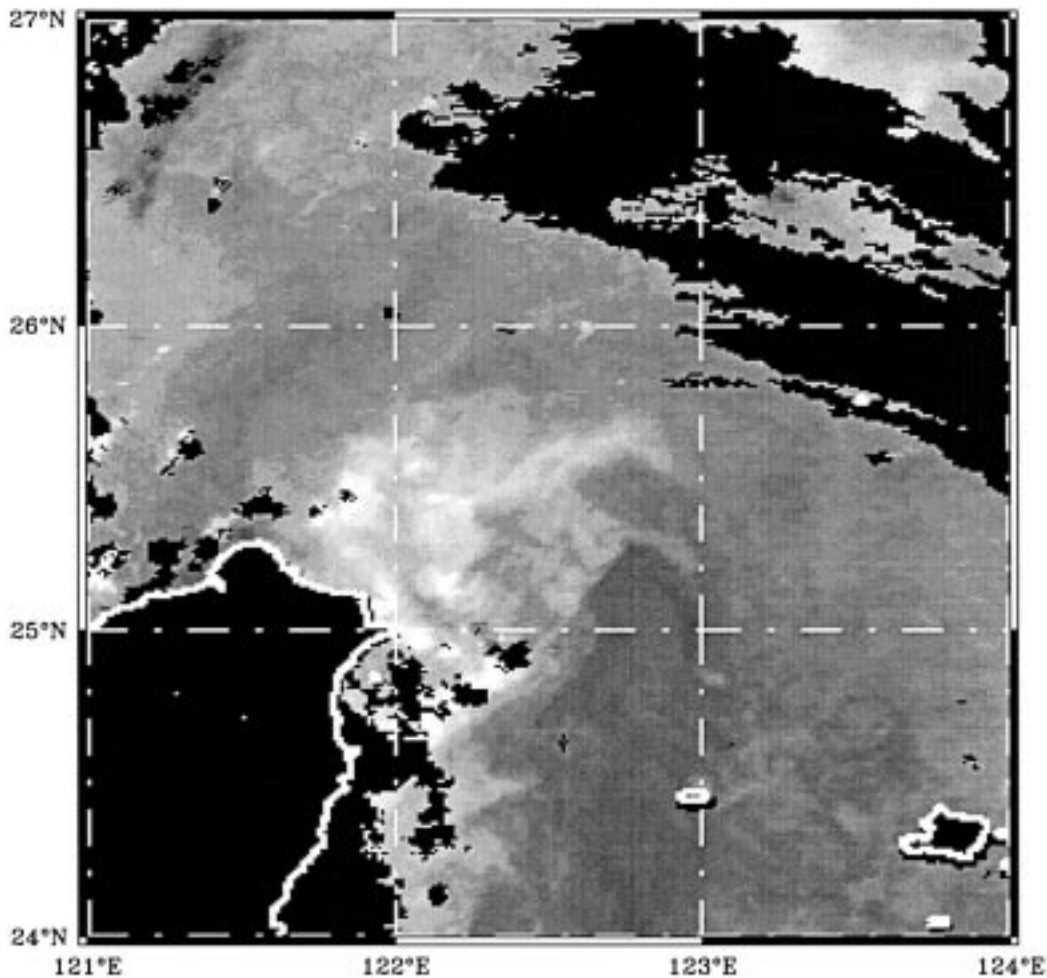
FIG. 6. Infrared image of the sea surface temperature in the study area obtained by NOAA-II on 12 August 1994. Light shading indicates low surface temperature.
