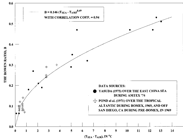
FIG. 1. A relationship between the Bowen ratio and sea–air temperature difference.
