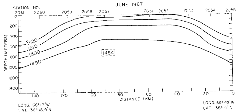
FIG. 2. Sound isovel section ( \text{m sec}^{-1} ) for cruise CF 156.
