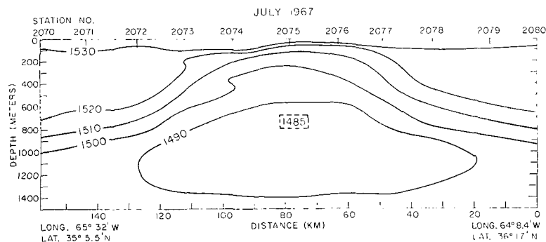
FIG. 3. Sound isovel section ( \text{m sec}^{-1} ) for cruise CF 158.
