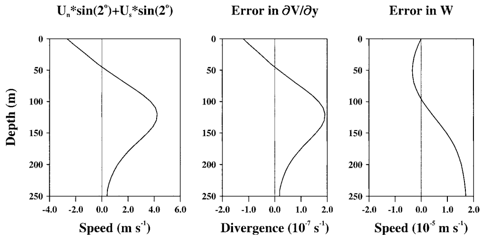
FIG. A2. Error profiles for \langle v\rangle , \partial\langle v\rangle/\partial y , and \langle w\rangle assuming systematic and oppositely directed 2° compass errors on each of the two off-equator moorings.
