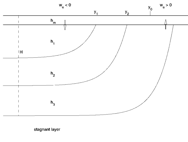
FIG. 10. Schematic representation of a model of the ventilated thermocline with three moving layers underneath a mixed layer with constant thickness. The variables h_m , h_1 , h_2 , and h_3 are the thicknesses of the individual layers, H is the thickness of the wind-driven gyre, and y_1 and y_2 are the subduction latitudes of layer 2 and 3, respectively. The latitude of zero vertical Ekman velocity ( w_e ) is marked by y_0 .
