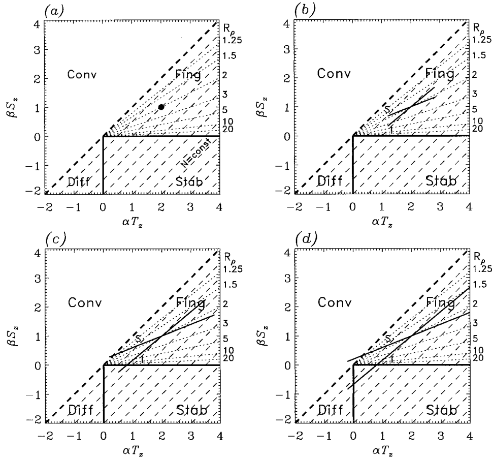
FIG. 6. Schematic depiction of intrusion growth on the (\alpha T_z, \beta S_z) plane, according to (5.1)–(5.2). Long-dashed lines denote constant N , and short-dashed lines constant R_\rho . Heavy lines separate fingering, convective, diffusive convective and stable regimes. (a) Initial conditions, lying close to background gradients, are denoted by the dot. (b) Growing intrusions describe line segments which lengthen in time. A line segment whose slope is less than R_\rho^{-1} is labeled by “S,” and one whose slope is greater than R_\rho^{-1} is labeled by “I.” (For intrusions to grow, this slope must lie between 0 and 1.) (c) As growth continues, I begins to penetrate the stable regime, and S the convective regime. (d) Still later, I penetrates the diffusive–convective regime as well. Intrusion I then consists of sequences of fingering, stable, diffusive convective, convective and fingering layers, whereas S consists of alternating fingering and convective layers.
