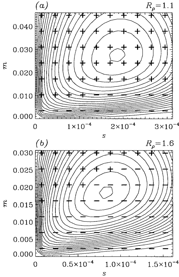
FIG. 10. Linear growth rate (units of N ) as a function of intrusion slope s and dimensionless vertical wave number m (units of [K_{\text{max}}/N]^{1/2} ). Plus signs indicate where criterion (5.10) for evolution toward staircases is satisfied. Minus signs indicate where evolution is toward conventional intrusions. In both cases, K_{\text{urb}} = 0.01 \text{ cm}^2 \text{ s}^{-1} , \Gamma_s = 5 \times 10^{-4} and the WR2 flux law is employed, with \text{Pr} given by (5.12) and \text{Pr}_0 = 10 : (a) R_\rho = 1.1 , maximum growth rate 2.66 \times 10^{-4} ; fastest-growing mode evolves toward a staircase; (b) R_\rho = 1.6 , maximum growth rate 0.75 \times 10^{-4} ; fastest-growing mode evolves toward conventional intrusions.
