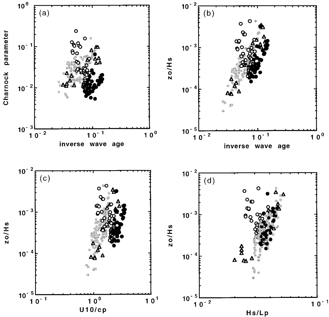
FIG. 3. Nondimensional roughness variables plotted against different scaling variables. Data are from HEXOS (small gray circles), AD96 (open triangles), and RASEX (open circles: U_{10m} < 10 \text{ m s}^{-1} , closed circles: U_{10m} > 10 \text{ m s}^{-1} ). Plots are (a) z_{ch} vs (c_p/u_{*k})^{-1} , (b) z_o/H_s vs (c_p/u_{*k})^{-1} , (c) z_o/H_s vs (c_p/U_{10m})^{-1} , and (d) z_o/H_s vs H_s/L_p .
