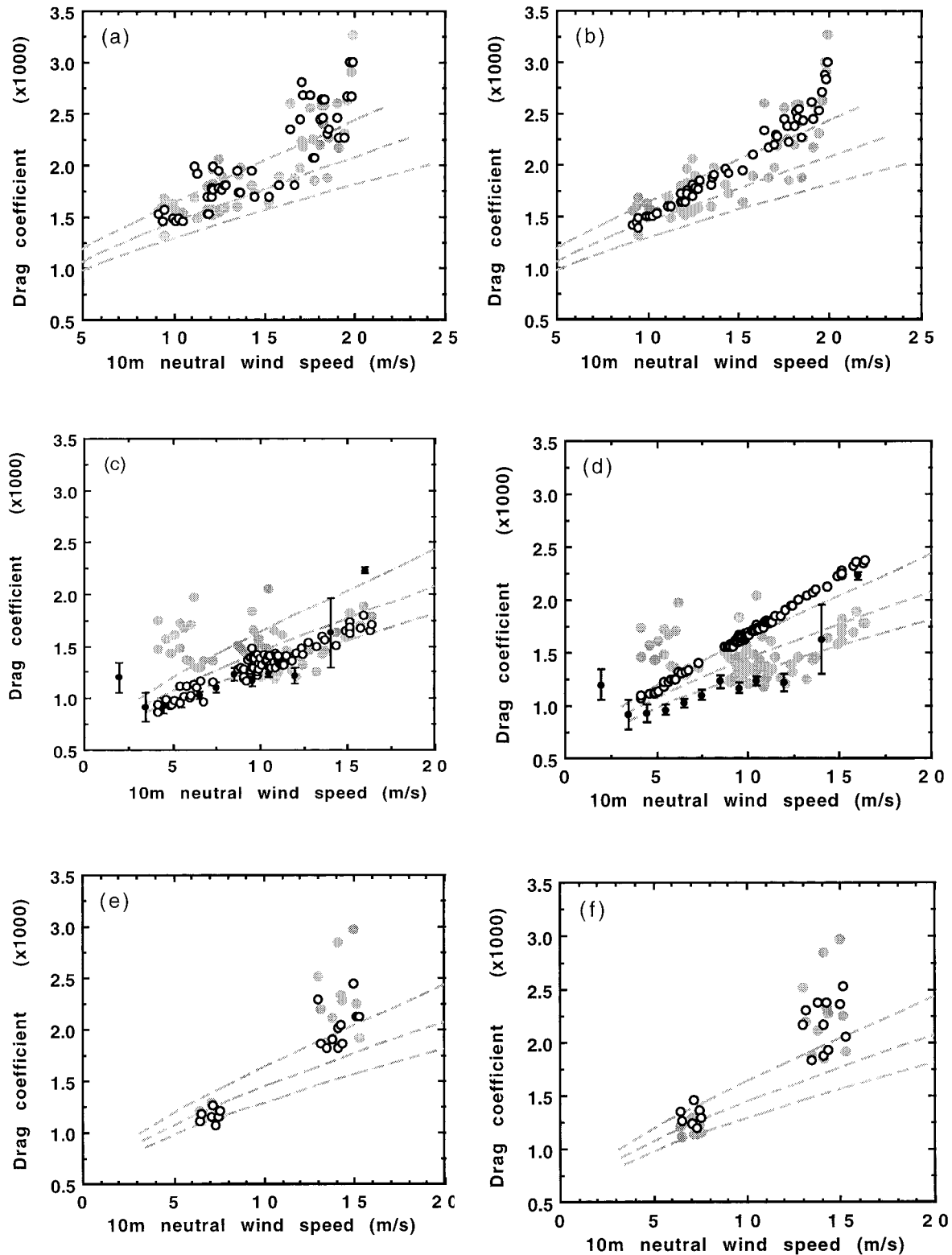
FIG. 5. Observed and calculated values of C_{D10m} for (top to bottom) HEXOS, RASEX, and AD96. Filled gray circles: the observations; open circles: values calculated from Eq. (6) (left plots) and from the Donelan (1990) formula (right plots). On the RASEX plots the gray circles are from JHVL98 and the points with error bars from VM97. The dashed lines show z_{ch} values of (bottom to top) 0.011, 0.018, and 0.030.
