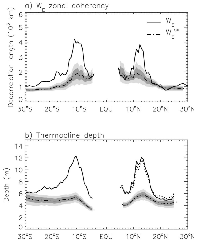
FIG. 7. (a) Comparison between the zonally averaged coherency of W_E (solid line), based on 6-yr low-pass filtered values, and the ensemble mean of the zonally averaged coherency of W_E^{\text{sc}} (dash-dot line). The ensemble contains 99 realizations of W_E^{\text{sc}} . Each W_E^{\text{sc}} field is obtained by randomly scrambling the monthly time series of W_E at each grid point. Decorrelation lengths were then calculated from the annually averaged scrambled time series. The dark shading indicates values of decorrelation lengths within 1 std dev from the ensemble mean, while the light shading shows values within 2 std dev from the ensemble mean. (b) Comparison between the zonally average standard deviation of thermocline depth obtained from the wave model forced by W_E and the ensemble mean of the zonally averaged standard deviation obtained with the W_E^{\text{sc}} fields. Values of thermocline depth standard deviation within 1 and 2 std dev from the ensemble mean are indicated by dark and light shading, respectively. The dot line in (b) shows the zonally averaged standard deviation of thermocline depth obtained with the modified forcing W_E^{\text{sym}} between 5° and 25°N.
