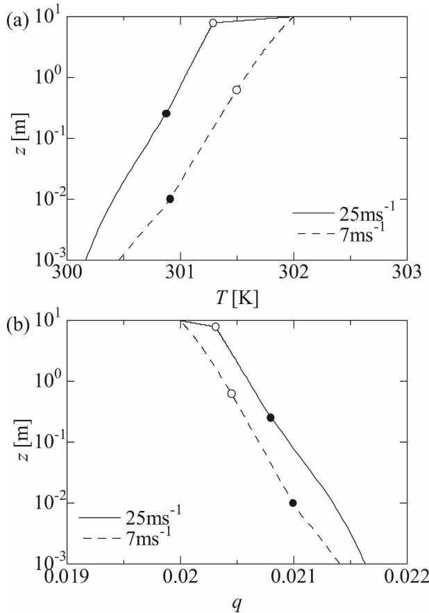
FIG. 3. (a) Vertical profiles of temperature and (b) specific humidity for u_{10} = 7 and 25 \text{ m s}^{-1} under a stably stratified condition, with T_w = 300 \text{ K} , t_{10} = 30 \text{ K} , \text{RH} = 80\% , and P_0 = 1000 \text{ hPa} . A black circle denotes the height of the top of the wave boundary layer; an open circle denotes the height of the top of the drop evaporation layer.
