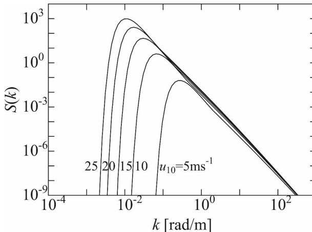
FIG. 1. Distributions of the omnidirectional spectrum S(k) for a mature sea for u_{10} = 5, 10, 15, 20, and 25 \text{ m s}^{-1} .
