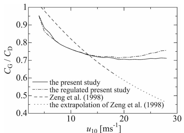
FIG. 6. Wind velocity dependence of C_G/C_D under an unstably stratified condition. The solid line denotes our result; the dashed line is the parameterization of Zeng et al. (1998); the dotted line is the extrapolation of the parameterization of Zeng et al.; and the chain line is our regulated result.
