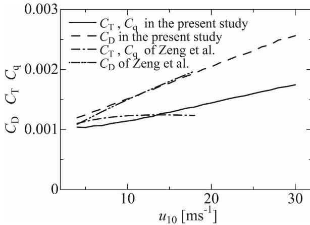
FIG. 2. Wind speed dependence of exchange coefficients C_D , C_T , and C_q for mature sea states obtained in the present study. Those reported by Zeng et al. (1998) are also shown. The solid line denotes C_T and C_q in the present study; the dashed line is C_D in the present study; the chain line is C_T and C_q of Zeng et al.; and the chain double-dashed line is C_D of Zeng et al.
