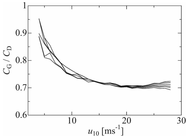
FIG. 7. Wind velocity dependence of C_G/C_D under unstably stratified conditions. The temperature difference T_w - T_{10} varies from 0.5 to 3.0 K, and the relative humidity varies from 0.7 to 0.9.
