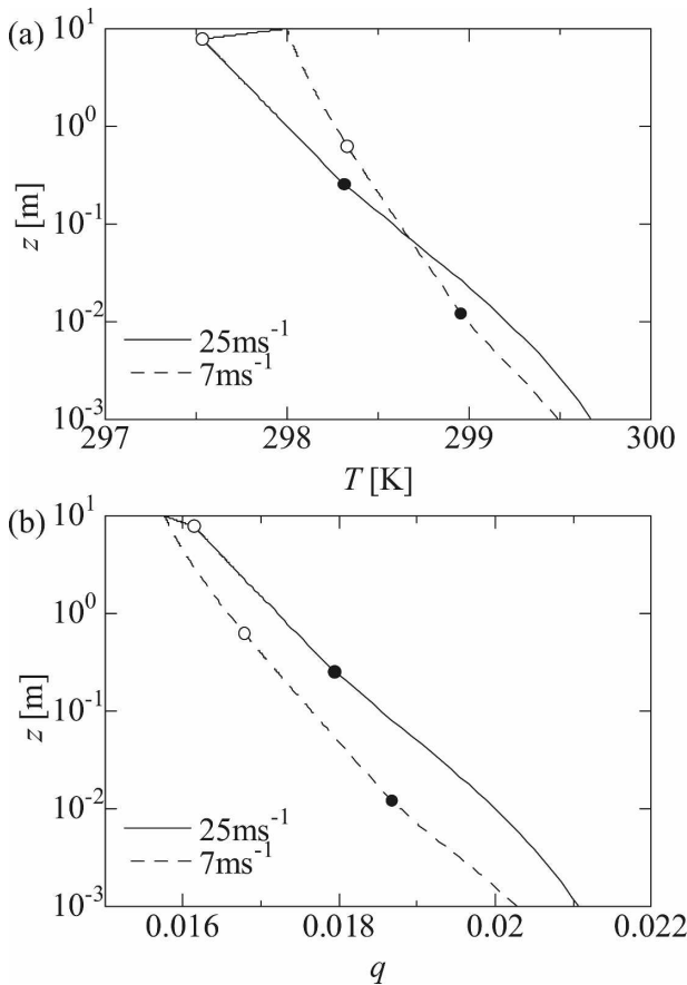
FIG. 4. (a) Vertical profiles of temperature and (b) specific humidity for u_{10} = 7 and 25 \text{ m s}^{-1} under an unstably stratified condition, with T_w = 300 \text{ K} , T_{10} = 298 \text{ K} , \text{RH} = 80\% , and P_0 = 1000 \text{ hPa} . A black dot denotes the height of the top of the wave boundary layer; an open circle denotes the height of the top of the drop evaporation layer.
