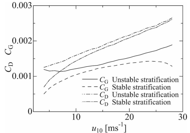
FIG. 5. Wind speed dependence of the exchange coefficient of total enthalpy C_G and the drag coefficient C_D under stably and unstably stratified conditions. The solid line denotes C_G under the unstably stratified condition; the dashed line is C_G under the stably stratified condition; the chain line is C_D under the unstably stratified condition; and the chain double-dashed line is C_D under the stably stratified condition.
