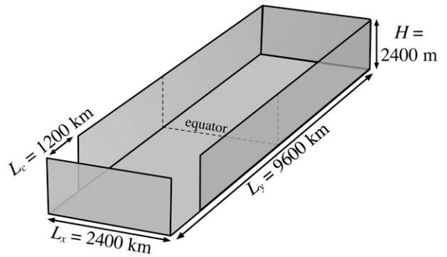
FIG. 2. The basin geometry of the numerical experiments. The horizontal resolution of the eddy-resolving and coarse-resolution models is 5.4 and 98 km, respectively. Both models use 20 unequally spaced vertical levels.
