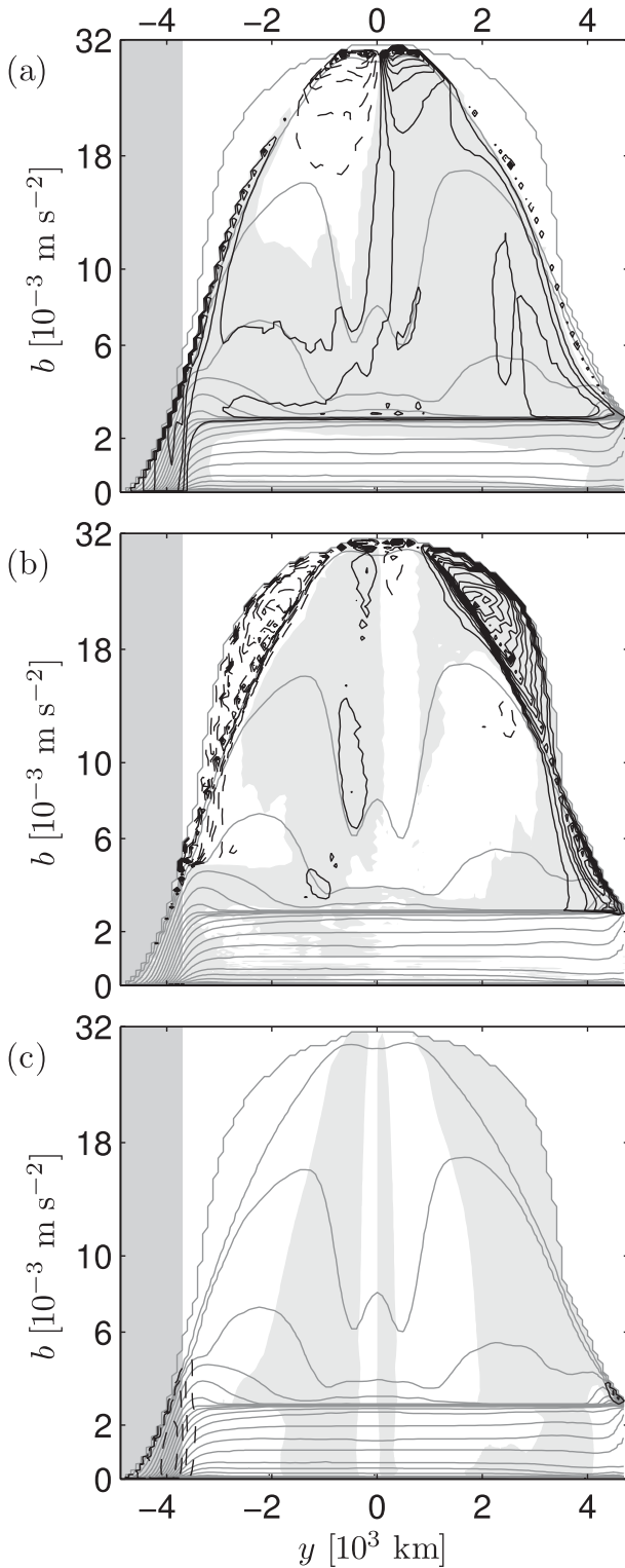
FIG. 7. (a) The zonally averaged component of the ROC shown in Fig. 5d, where the zonal average is performed at fixed z levels as a function of y and b . (c) The portion of the transport due to the modified Gent–McWilliams parameterization and (b) the remainder, which is associated with flows with zero zonal average that are resolved by the computation (i.e., gyres, large-scale waves, and
