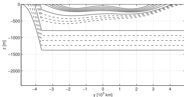
FIG. 8. The buoyancy field \bar{b}(y, \bar{z}) obtained as a solution to (27) with \psi given by (28). The contour interval is as in Figs. 3a–c. The solution is omitted for those contours outcropping more than twice, because the expression (28) is not valid in that case.
