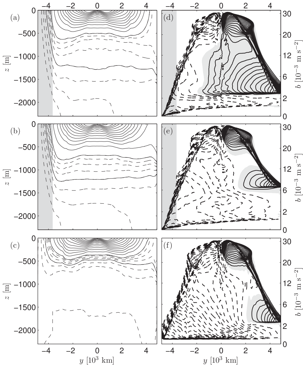
FIG. 3. (a) The zonal- and time-averaged buoyancy as a function of y and z for the control and (d) the ROC as a function of y and b for the control. The reentrant channel is shaded. Note the strong pole-to-pole ROC and the strong deep stratification. (b),(e) All parameters are identical to the control, but the surface buoyancy in the NH is increased so that there are no shared outcropping values between the NH and the channel. (e),(f) All parameters are identical to the control, but the channel is closed. The contour intervals for (a)–(c) are 2 \times 10^{-3} \text{ m s}^{-2} (solid) and 5 \times 10^{-4} \text{ m s}^{-2} (dashed). The contour interval for (d)–(f) is 0.5 Sv. Positive values are solid, negative values are dashed, and the area of positive contours is shaded.
