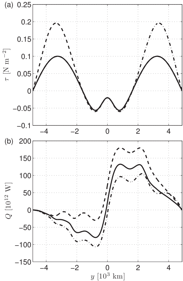
FIG. 4. (a) Zonal wind stress \tau and (b) meridional heat transport Q for the control (solid), increased southern wind (dashed), and increased northern wind (dashed–dotted) experiments.
