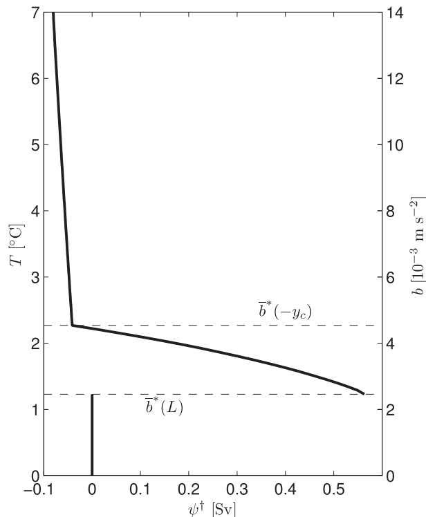
FIG. 9. ROC \psi(b) corresponding the buoyancy field shown in Fig. 8. The values of the surface buoyancy profile b^* at the northern boundary, y = L , and the northern edge of the channel, y = -y_c , are indicated.
