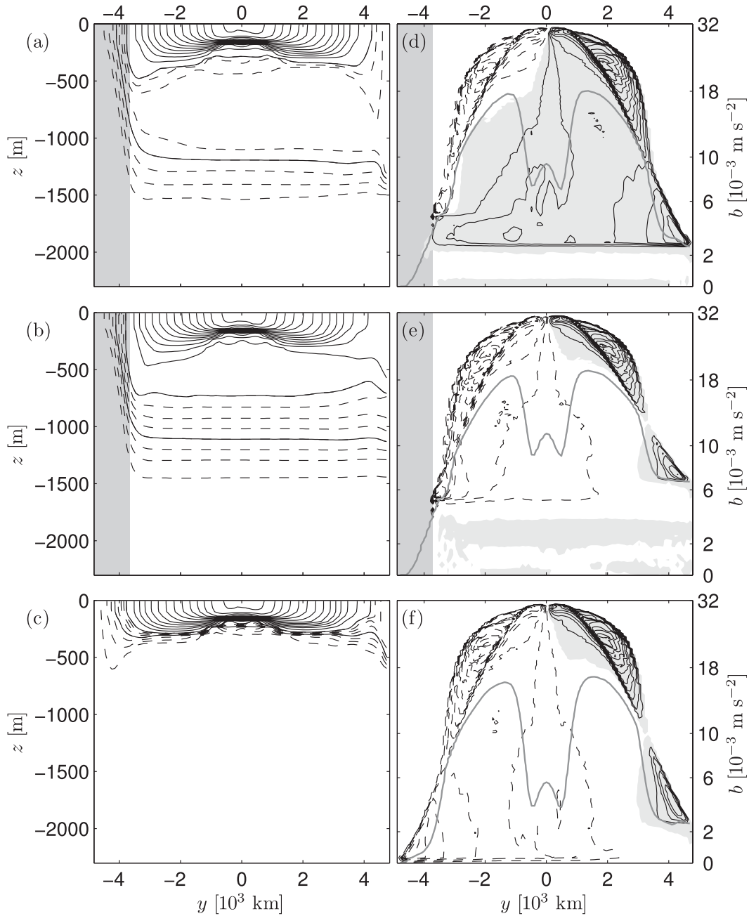
FIG. 5. As in Fig. 3, but for the coarse-resolution model. The contour intervals are as in Fig. 3. The thick gray line gives the position of the base of the mixed layer in buoyancy coordinates.
