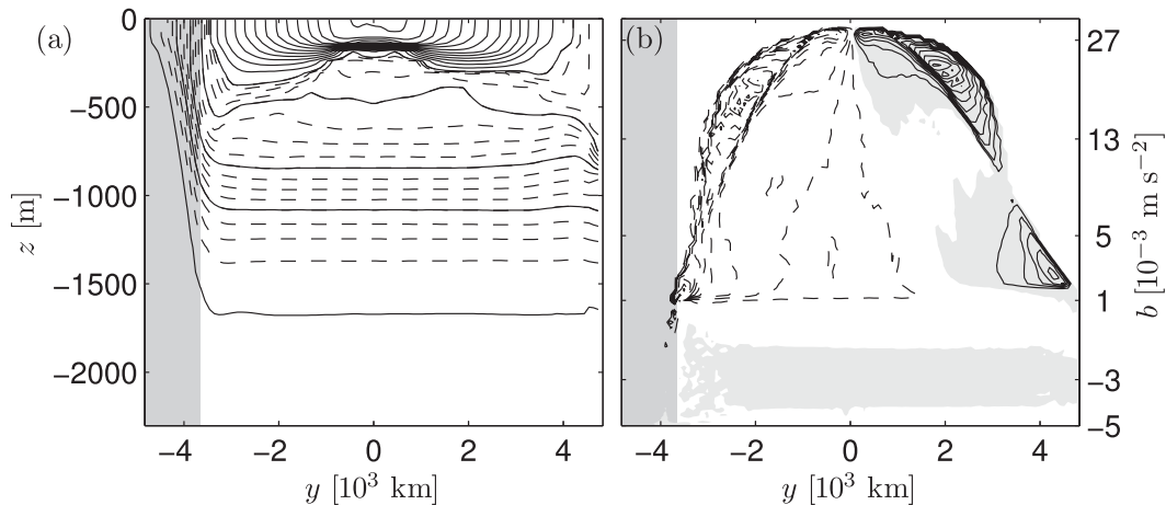
FIG. 6. As in Fig. 5 (top) except that the surface buoyancy forcing is given by (7). The contour intervals are as in Fig. 5.
