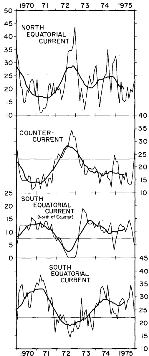
FIG. 8. Time series of sea level differences (cm) across zonal currents in the central equatorial Pacific, 1970-75. The thin curves give monthly averages, the heavy curves the 12-month running means.
