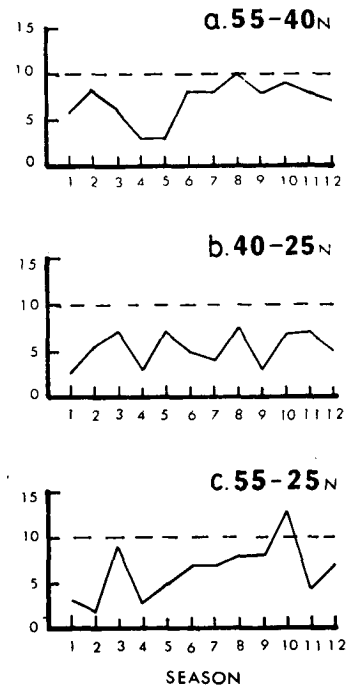
FIG. 7. As in Fig. 4 except abscissa is the season type and ordinate is the frequency of collocation of maximum negative ΔSSTA and maximum northerly VgA.
