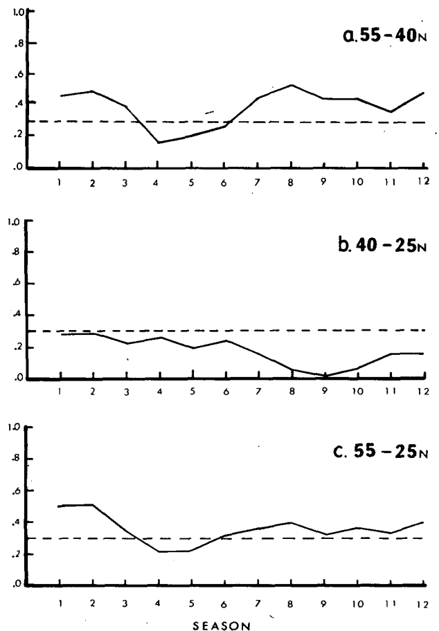
FIG. 9. As in Fig. 8 except abscissa is the season type. Plots were made at the end month of the three months used to define the seasonal mean.
