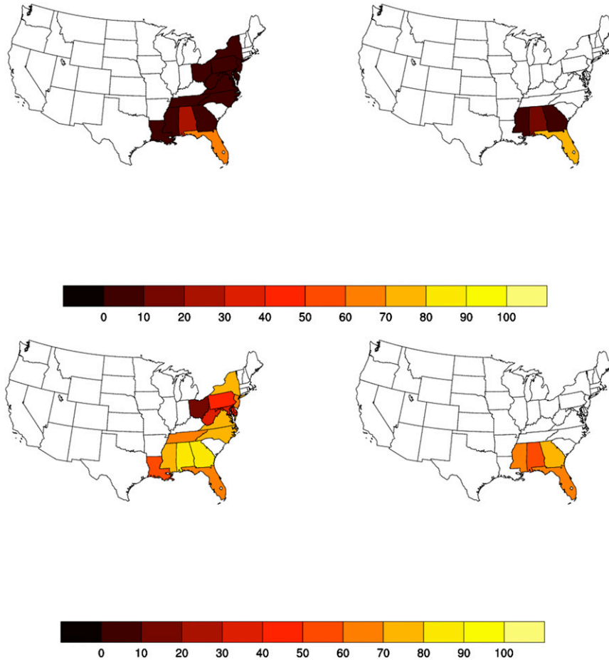
FIG. 1. (a) PCS state losses as a percent of storm total loss for (left) Ivan and (right) Dennis. (b) PCS state personal business line losses as a fraction of total state loss for (left) Ivan and (right) Dennis.
