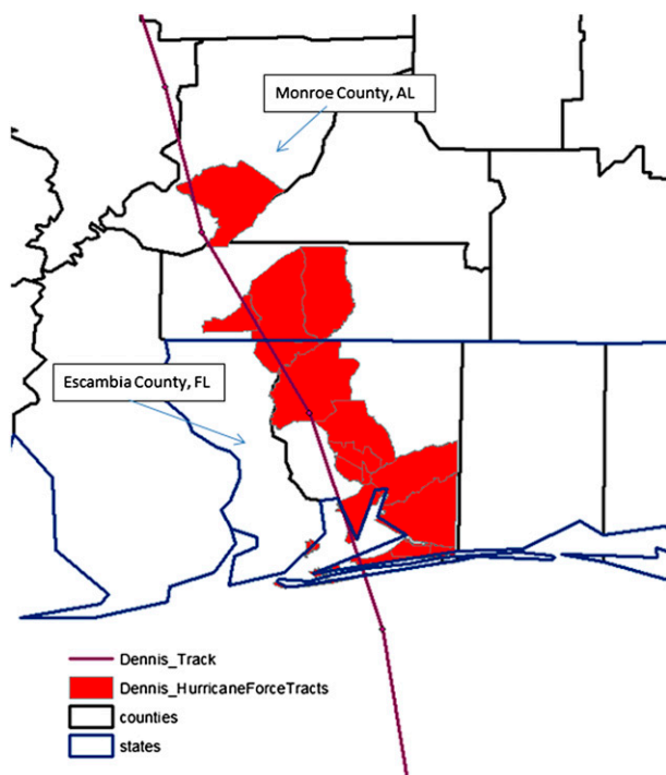
FIG. 3. Hurricane Dennis hurricane force census tracts by county and state.
