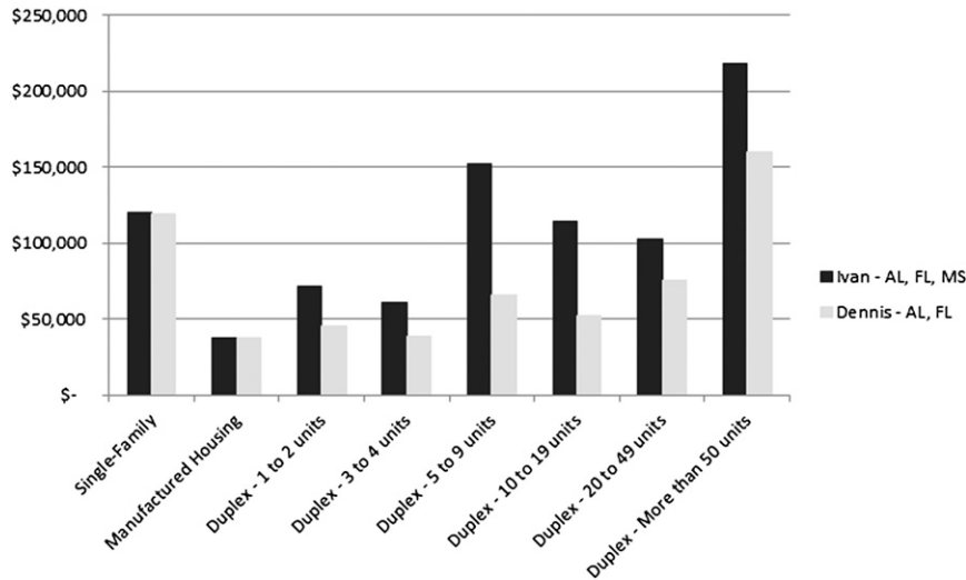
FIG. 5. Average residential building values per hurricane force impacted tracts.
