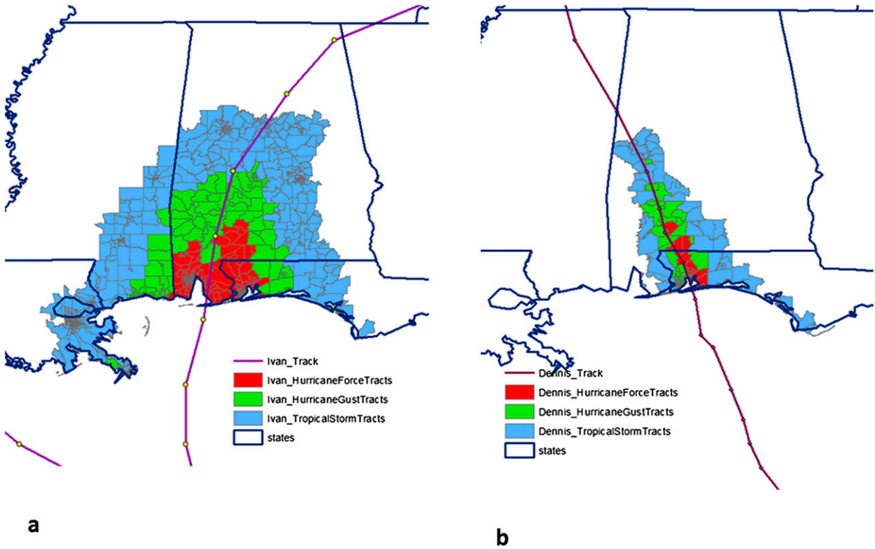
FIG. 2. (a) Hurricane Ivan impacted geographical areas. (b) Hurricane Dennis impacted geographical areas.
