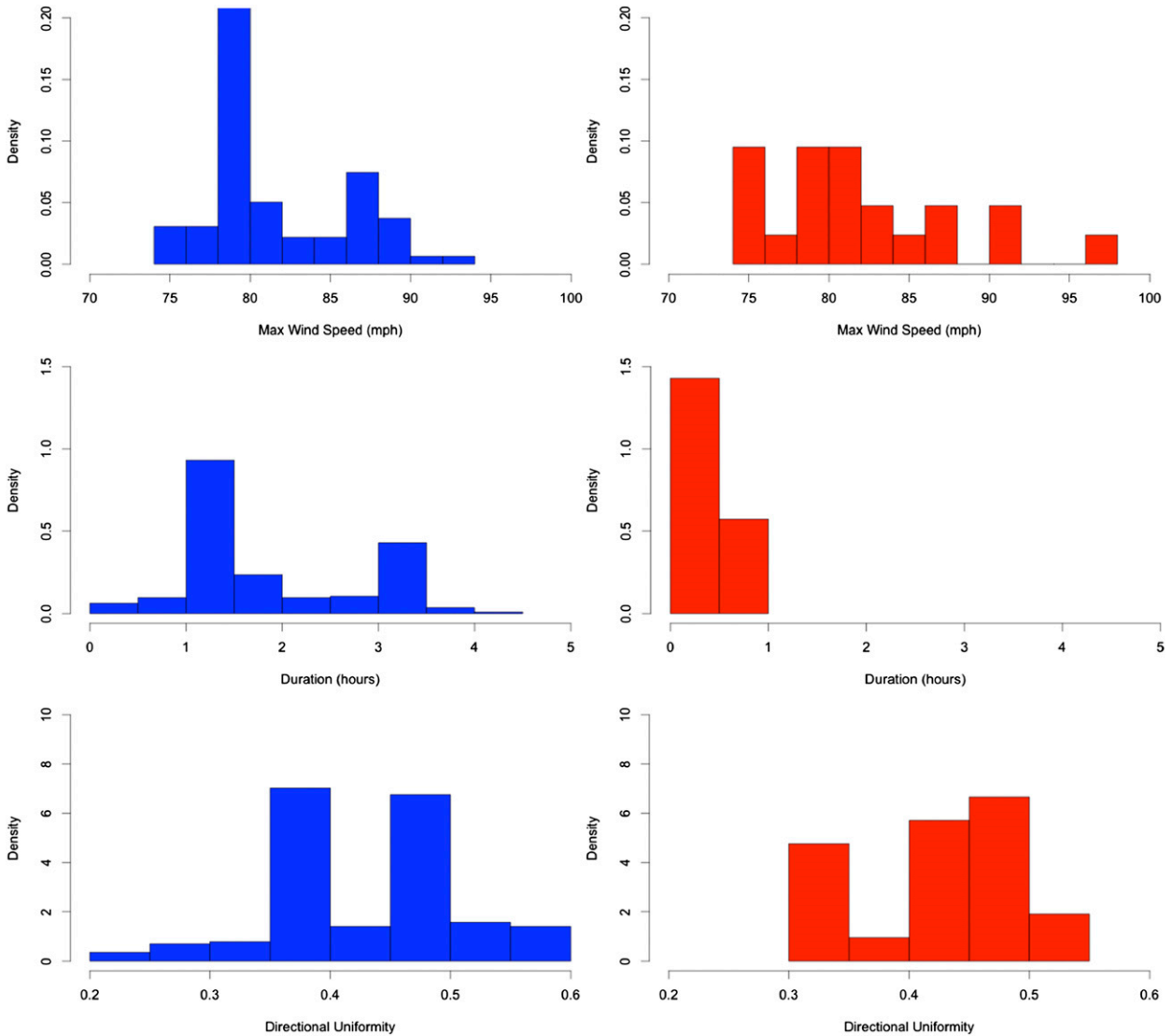
FIG. 4. Distribution of census tract average (a) maximum wind speeds, (b) duration of hurricane force winds, and (c) directional uniformity for census tracts impacted by Ivan’s hurricane force winds (data source: H*Wind; Powell et al. 1998).
