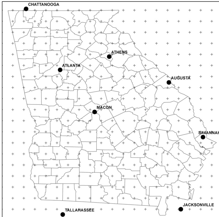
FIG. 1. Locations of surface-observing stations where data for computing AT were obtained. Crosses represent a 0.25^\circ \times 0.25^\circ interpolated grid of AT values.
