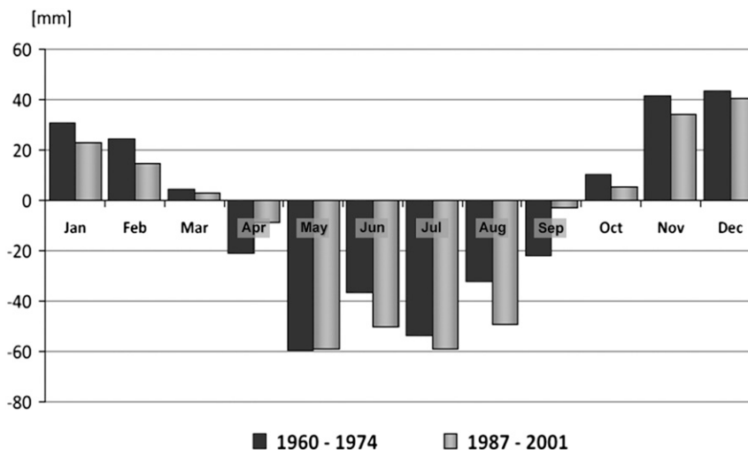
FIG. 5. Climatic water balance trends in the study area. Source: Stagl and Hattermann (2011) (with permission).
