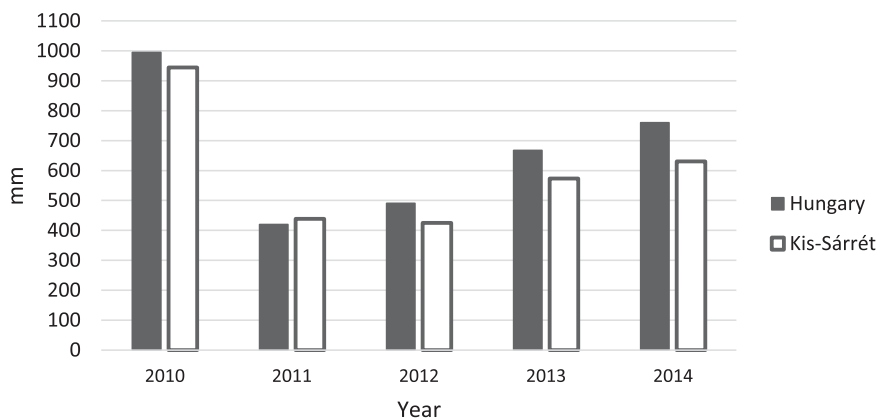
FIG. 2. Average annual precipitation in Hungary and the study area from 2010 to 2014. Source: Hungarian Meteorological Service.
