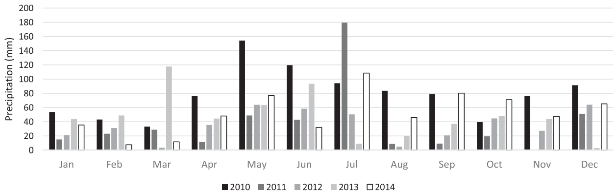
FIG. 4. Average monthly precipitation in the Kis-Sárrét area from 2010 to 2014. Source: Hungarian Meteorological Service, Körösszakál station.
