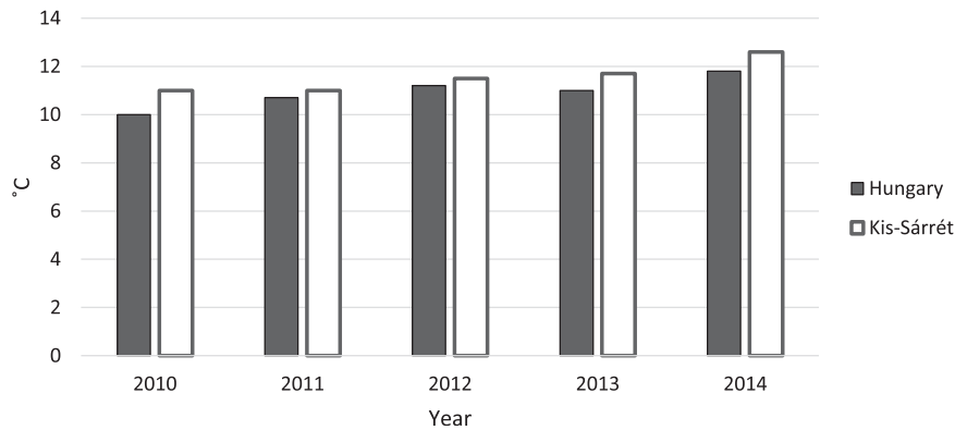
FIG. 1. Average annual temperature in Hungary and the study area from 2010 to 2014. Source: Hungarian Meteorological Service.
