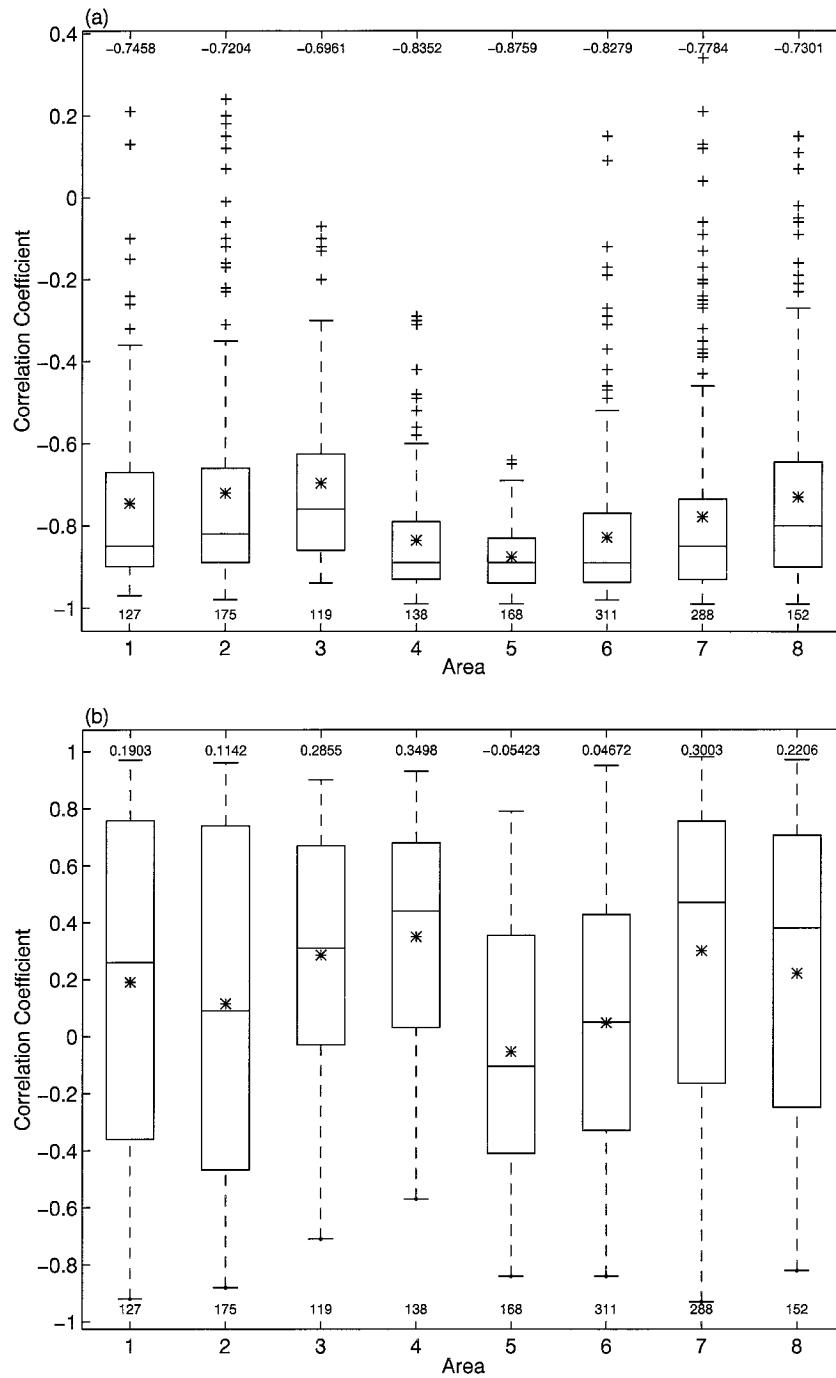
FIG. 13. As in Fig. 6 except for (a) DTR MSU3 T_b and 500-mb height correlation coefficients, and (b) DTR MSU3 T_b and 500-mb height correlation coefficients, and for only those times when TC \geq 0.80 .
