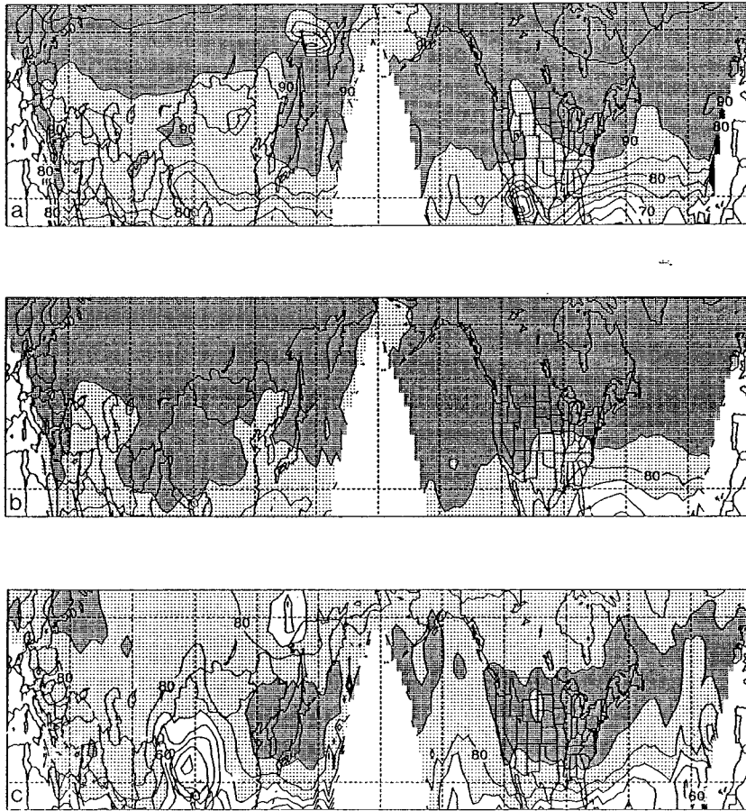
FIG. 8. Analysis of (a) UF, (b) 14-day LP filtered, and (c) 5-day HP filtered 6-month temporal correlation coefficients (solid, contour interval 10^{-2} ) between the MSU3 T_b and 400–100-mb thickness.
