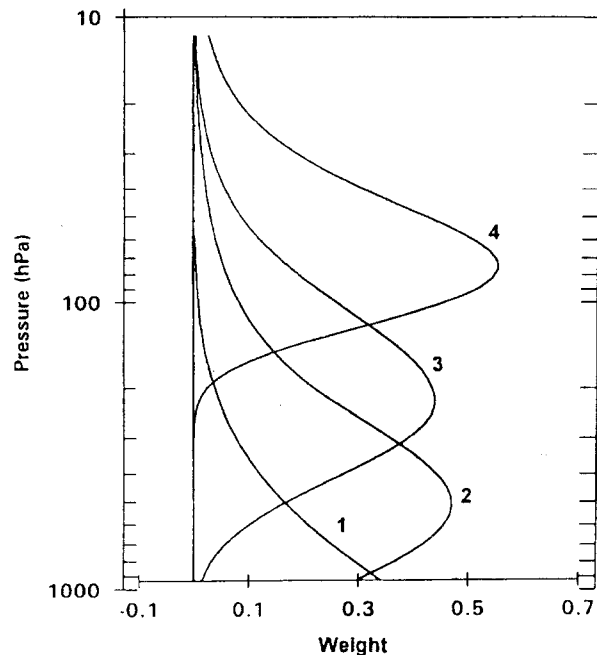
FIG. 1. Vertical profile of weighting functions for MSU channels 1–4. The weight equals the change of transmittance with \log_e(p) . From Spencer et al. (1995).
