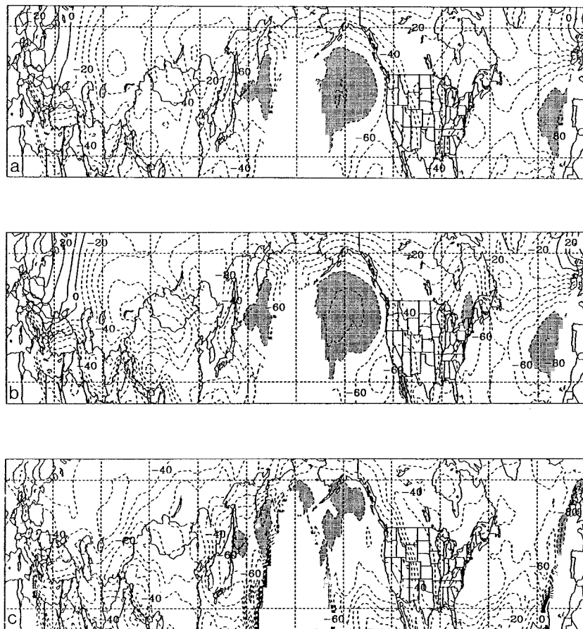
FIG. 17. As in Fig. 8 except for MSU3 T_b and sea level pressure correlation coefficients.
