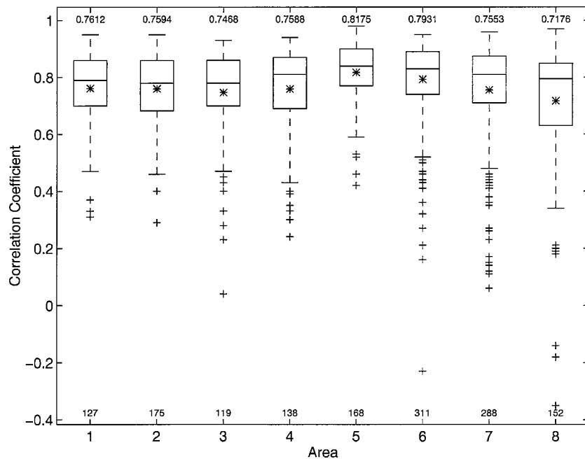
FIG. 9. As in Fig. 6 except for DTR MSU3 T_b and 200-mb temperature correlation coefficients and for only those map times when TC \geq 0.80.
