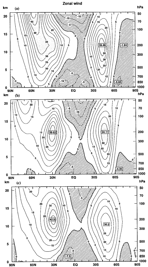
FIG. 3. Same as in Fig. 2 except for zonally averaged monthly mean wind from 1000 to 50 mb.
