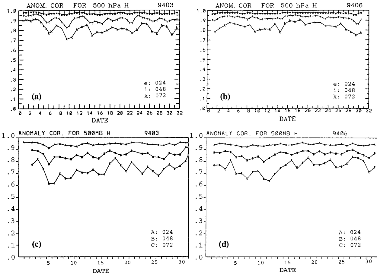
FIG. 7. The 500-mb height anomaly correlation for the Northern Hemisphere (20°–80°N) of 24-, 48-, and 72-h operational forecasts by (a) the second-generation GFS in March 1994, (b) the second-generation GFS in June 1994, (c) the first-generation GFS in March 1994, and (d) the first-generation GFS in June 1994. The anomaly correlation is computed by correlating the forecast anomaly to their own analyzed anomaly.
