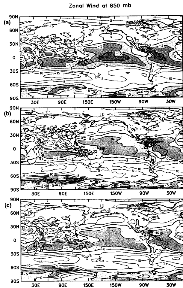
FIG. 5. Same as in Fig. 4 except for zonal wind at 850 mb.
