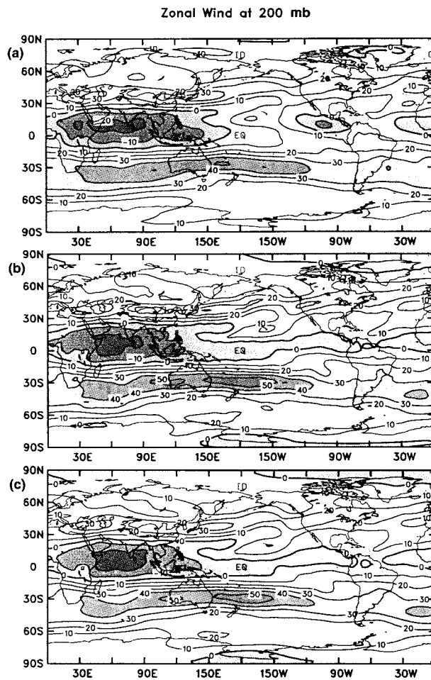
FIG. 4. Fifteen-day (1–15 July 1994) mean zonal wind at 200 mb from (a) the second-generation GFS analysis with real observations operationally received at the CWB only, (b) the ECMWF analysis, and (c) the second-generation GFS analysis with the real observations plus the supplemental observations from the 2.5° ECMWF analysis at 850, 500, and 200 mb.
