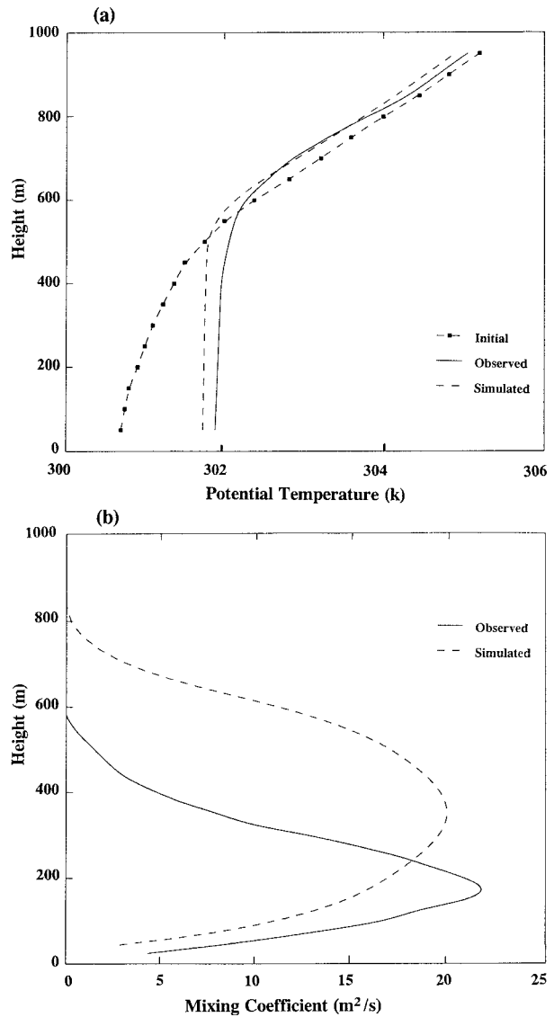
FIG. 1. Boundary layer profiles (observed (solid) and simulated (dashed) by the one-dimensional PBL model with 600-s time steps and four vertical layers in the bottom 400 m: (a) potential temperature and (b) eddy mixing coefficient for momentum. The dotted lines are initial values for the model simulation.
