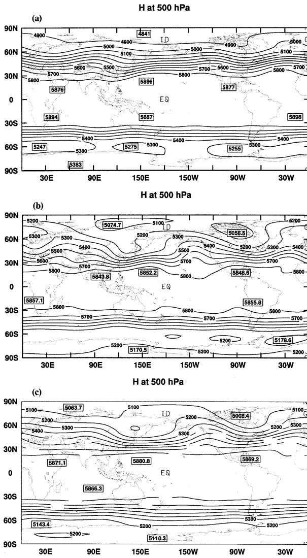
FIG. 2. Monthly mean 500-mb height in January from the T47 second-generation GFS climate simulation (a) without and (b) with the gravity wave drag parameterization, and (c) the corresponding 10-yr mean analysis from NCEP.
