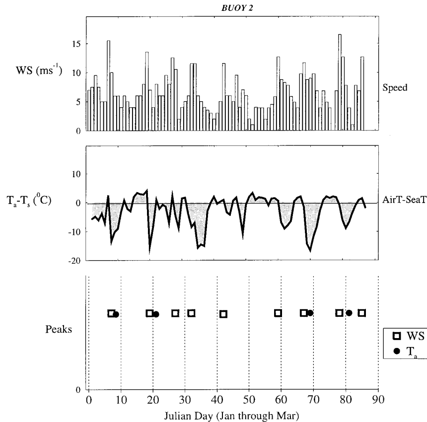
FIG. 4. Time series of wind speed (WS) in \text{m s}^{-1} (top) and air-sea temperature difference ( T_a - T_s ) in ^{\circ}\text{C} (middle) at buoy 2 from January through March 1996. (Bottom) Open squares indicate cases when only peaks in wind speed occurred, and filled circles when significant peaks of both wind speed and air temperature occurred simultaneously.
