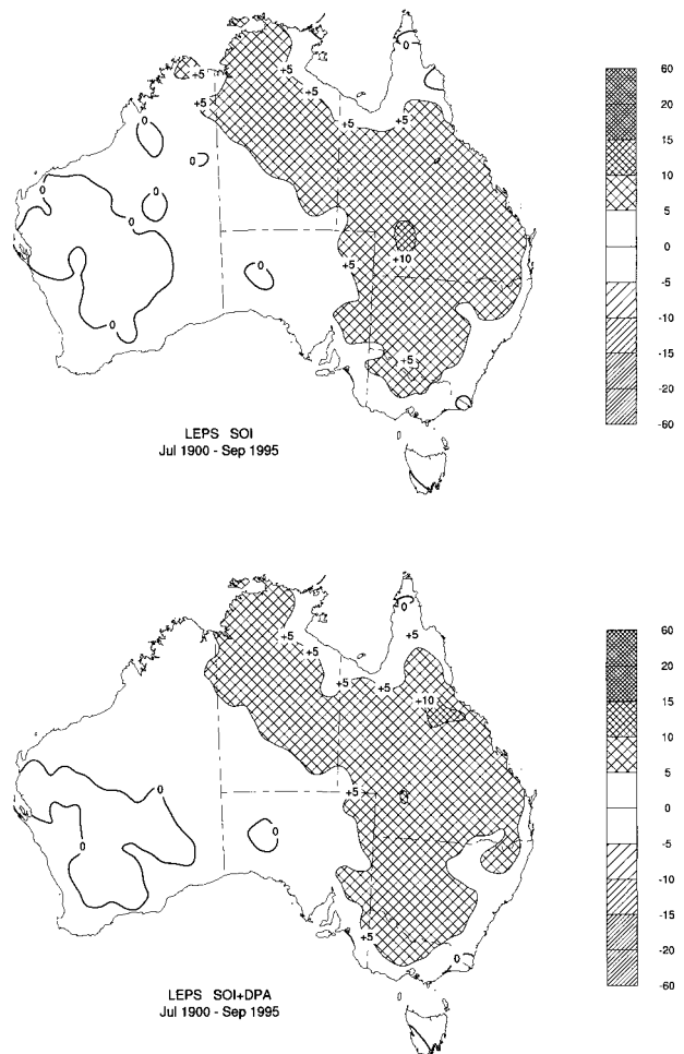
FIG. 7. Comparison of LEPS scores for SOI phase model (SOI) hindcasts for 1900–95 Australian winter rainfall with those from the combination of SOI phase model and a Darwin pressure phase model.
