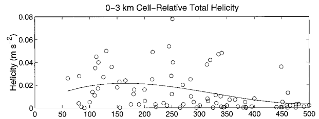
FIG. 14. Distribution of the cell-relative total helicity as a function of radial distance from storm center. The plotting convention is the same as in Fig. 3b.
