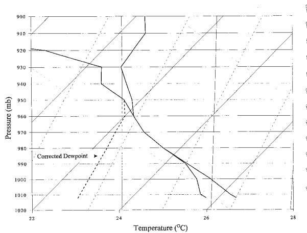
FIG. 1. Skew T - \log p plot of ODW 3476 dropped in Gustav at a radius of 325 km. The bold solid lines show temperature and dewpoint, and the bold dashed line is the corrected dewpoint. Pressure in mb is shown by the thin horizontal lines, temperature lines are the thin solid lines that run from lower left to upper right, adiabats are light dotted lines running from lower right to upper left, mixing ratio lines are dashed, and the moist adiabats are vertical solid lines. Wind barbs are shown at right and follow standard notation. Mixing ratio lines are plotted every 2 \text{ g kg}^{-1} starting with 22 \text{ g kg}^{-1} .
