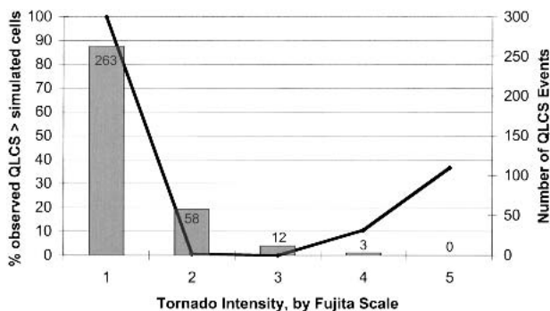
FIG. 4. Histogram of 1998–2000 U.S. QLCS tornado distribution by F scale, and percentage of the 10 000 Monte Carlo realizations in which there were more observed QLCS tornadoes in an F-scale bin than there were simulated (cell) tornadoes. Realizations are based on 336 cell tornadoes, which excludes F0 cell tornadoes.
