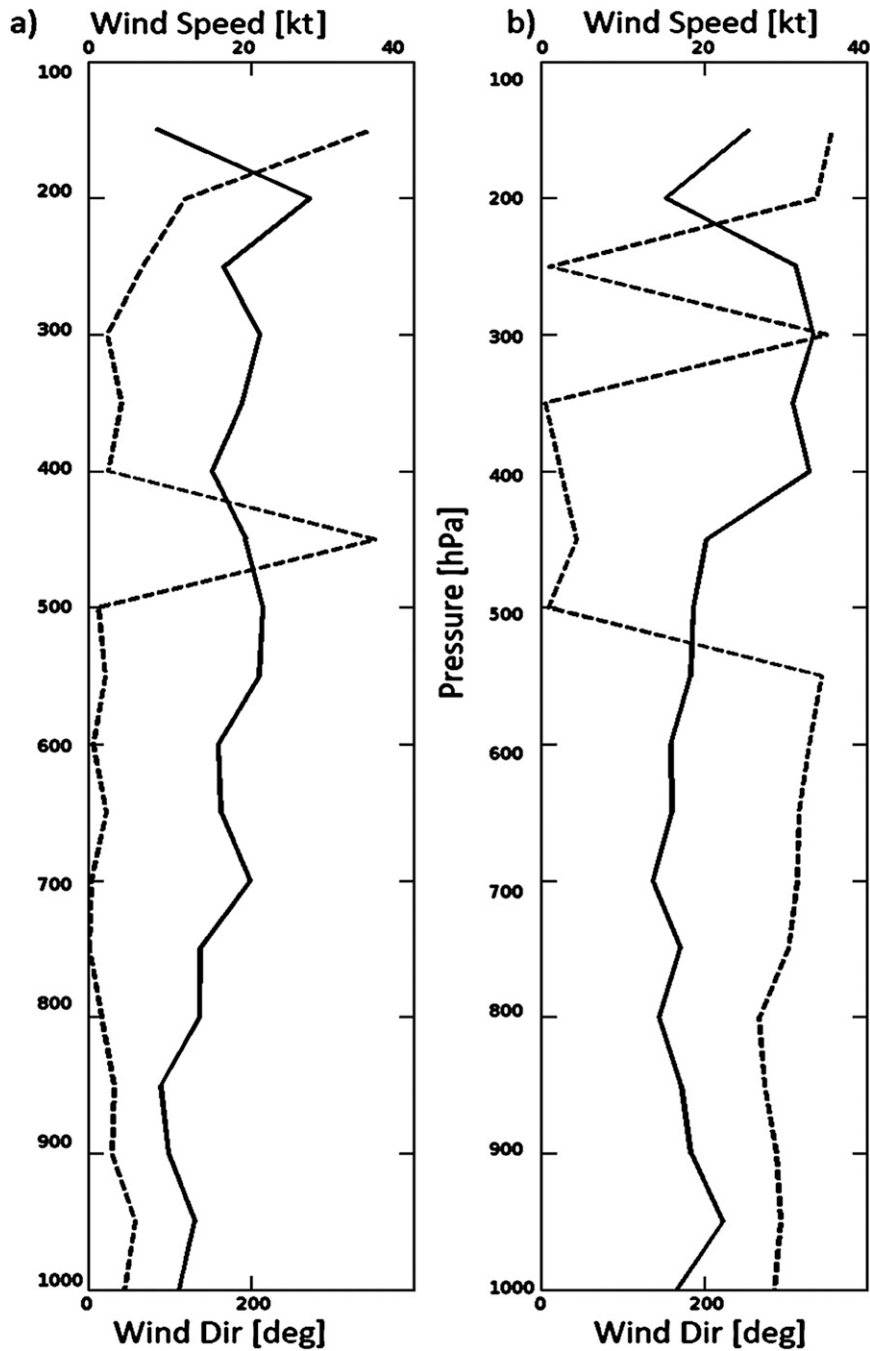
FIG. 4. Vertical profiles of wind speed (solid) and direction (dashed) produced by two sondes selected from the plot in Fig. 3 [points (a) and (b)].
