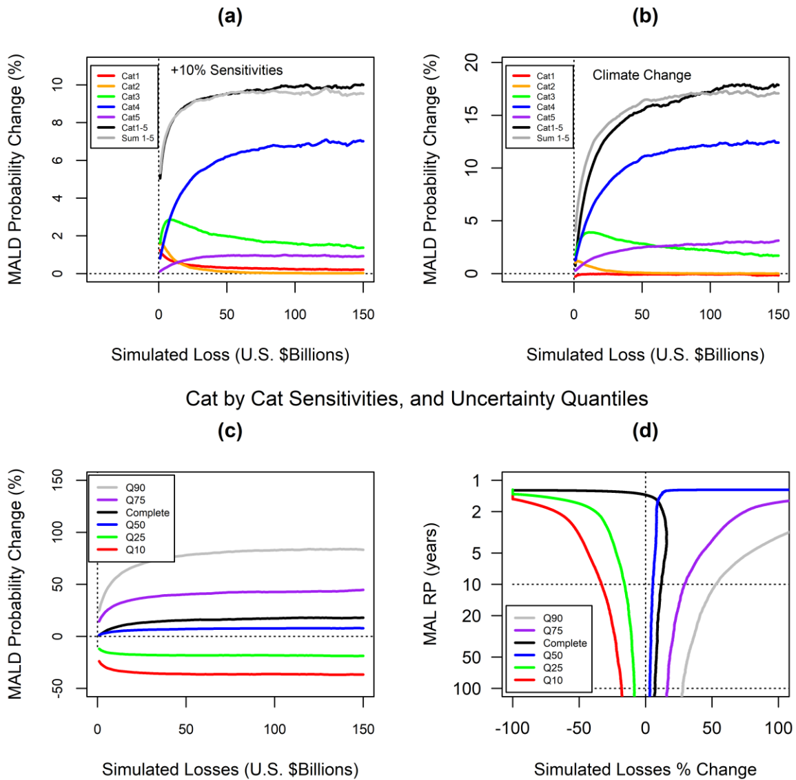
Figure S3: As figure 7, but for the MALD.
