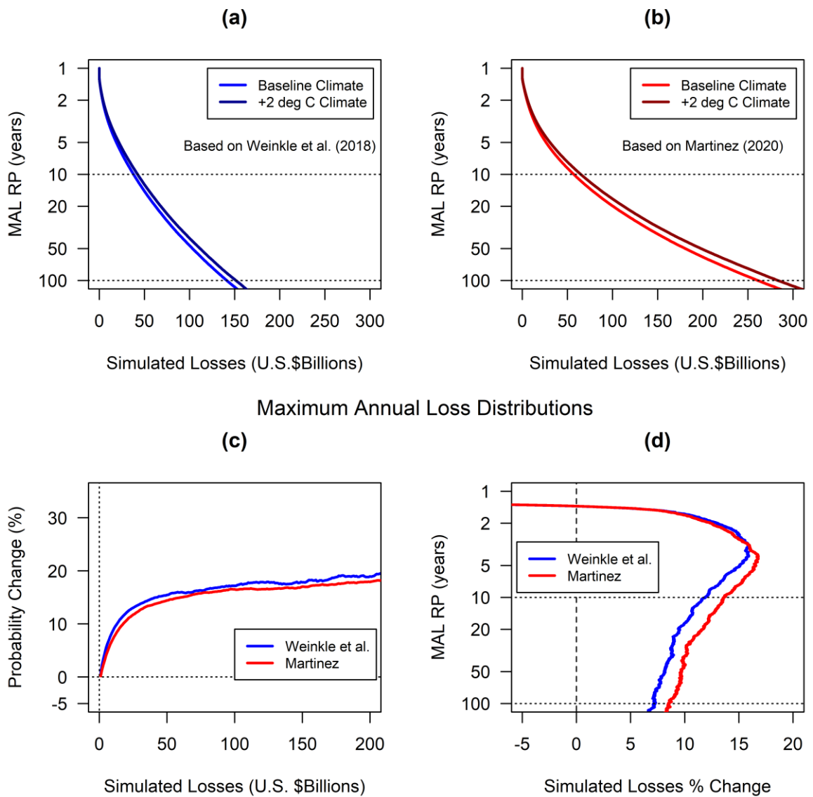
Figure S1: As figure 5, but for the MALD.
