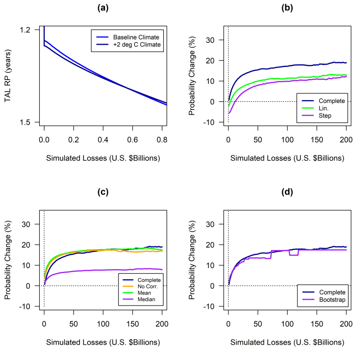
Figure S2: As figure 6, but for the MALD.
