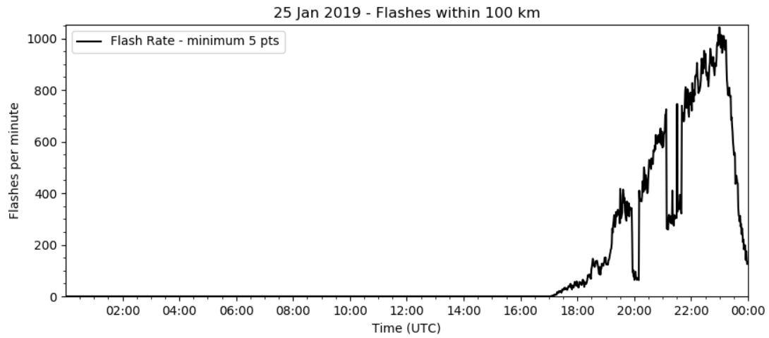
Figure S1. One-minute LMA flash rate time series (minimum 5 sources per flash), within 100 km of the network, for 25 January 2019.
