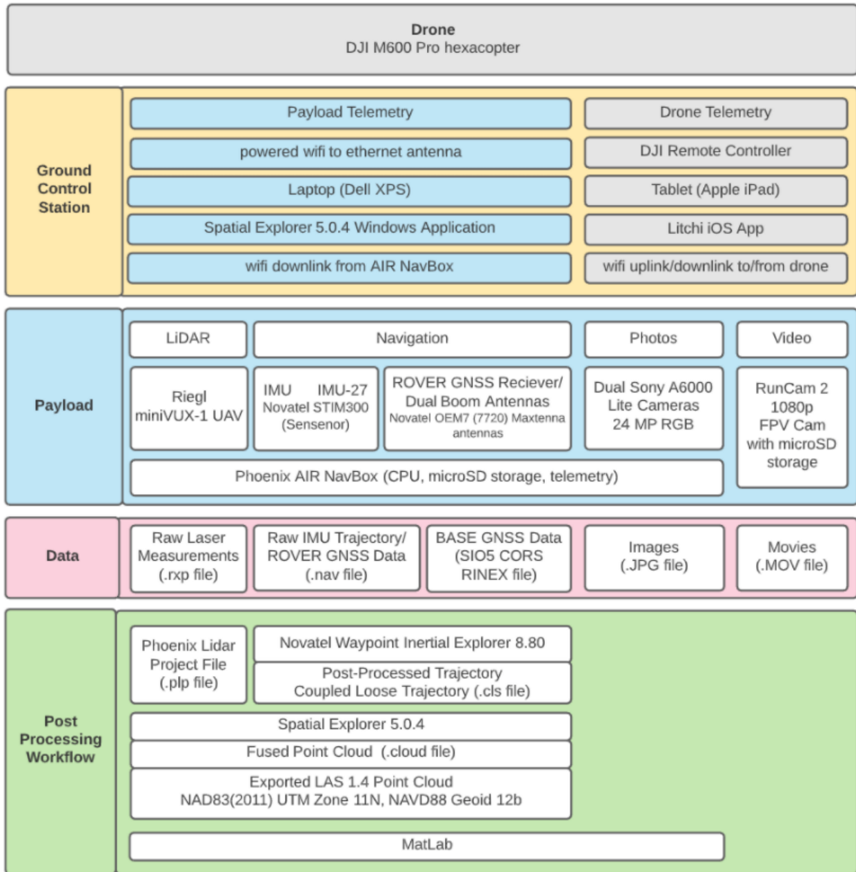
Supplemental Figure: Schematic of workflow for acquiring LiDAR data with Pheonix miniRANGER-LITE on the DJI M600 Pro Hexacopter.
