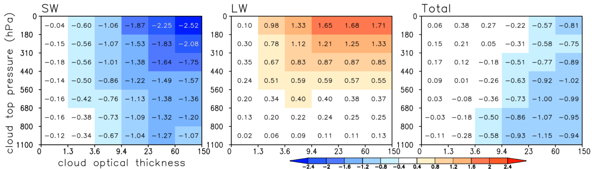
Figure S1. Ocean-only globally and annually-averaged shortwave, longwave, and total radiation “pseudo-CRks” derived from the CERES FluxByCldTyp product for the year 2007. These pseudo-CRks are multiplied with the binned CFs in the joint histograms of Fig. 6 to obtain distributions of CREs in the CTP-TAU phase space (Fig. 12).
