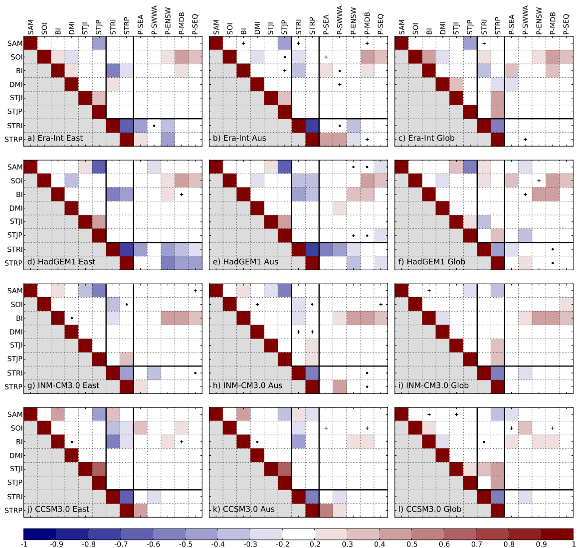
Fig. S 4: As in Fig. 1 but for Austral winter (JJA) in CMIP3.
