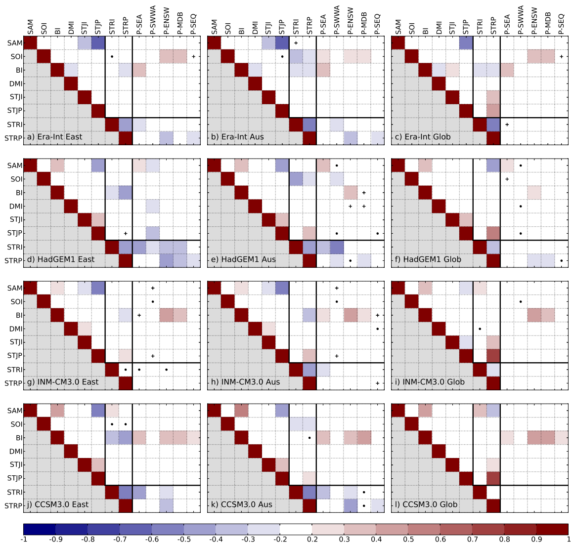
Fig. S 7: As in Fig. 1 but for Austral autumn (MAM) in CMIP3.
