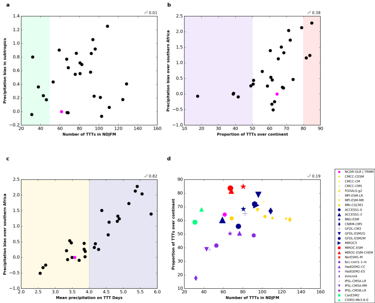
Figure S1: As Figure 8, but with the Outgoing Longwave Radiation (OLR) threshold set at 5 \text{ Wm}^{-2} lower than that used in the paper.
