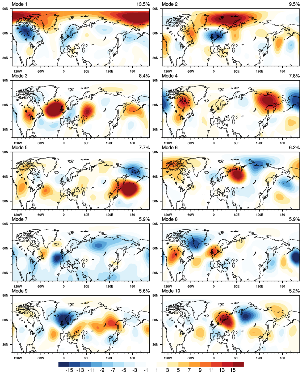
Figure S1. The 10 leading patterns and associated time series for the entire period (1973–2012), obtained from the rotated empirical orthogonal function (REOF) analysis to high summer (July–August) mean 500-hPa geopotential height anomalies, following the definition of Barnston and Livezey (1987).
