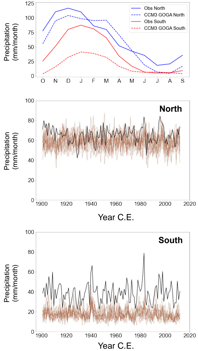
Figure S1: Same as Figure 1 in the paper, but for the CCM3 GOGA ensemble.
