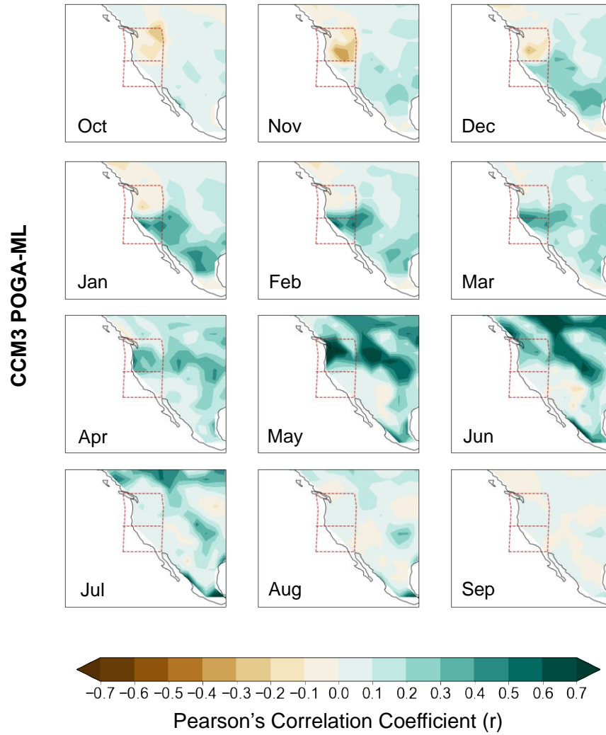
Figure S4: Same as Figure 2 in the paper, but for the CCM3 POGA-ML ensemble.
