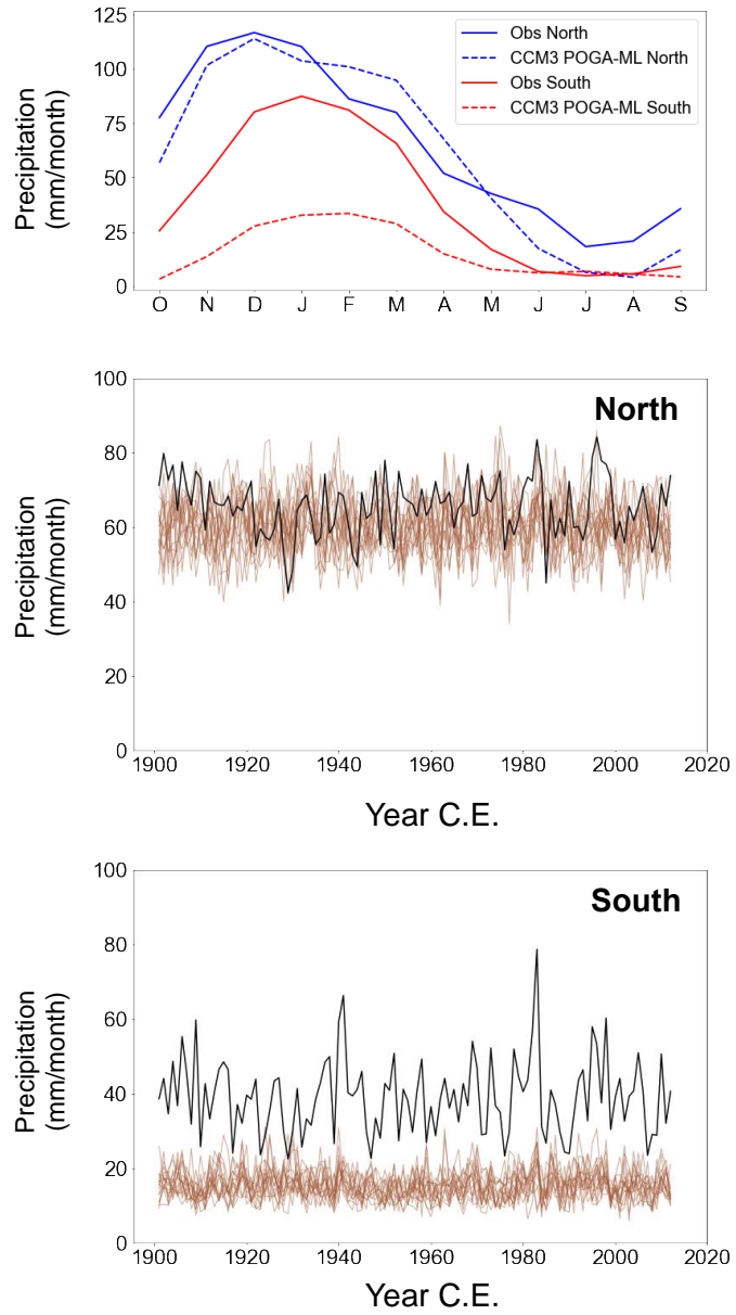
Figure S2: Same as Figure 1 in the paper, but for the CCM3 POGA-ML ensemble.
