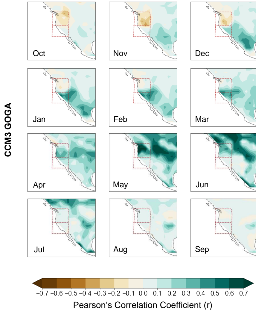
Figure S3: Same as Figure 2 in the paper, but for the CCM3 GOGA ensemble.
