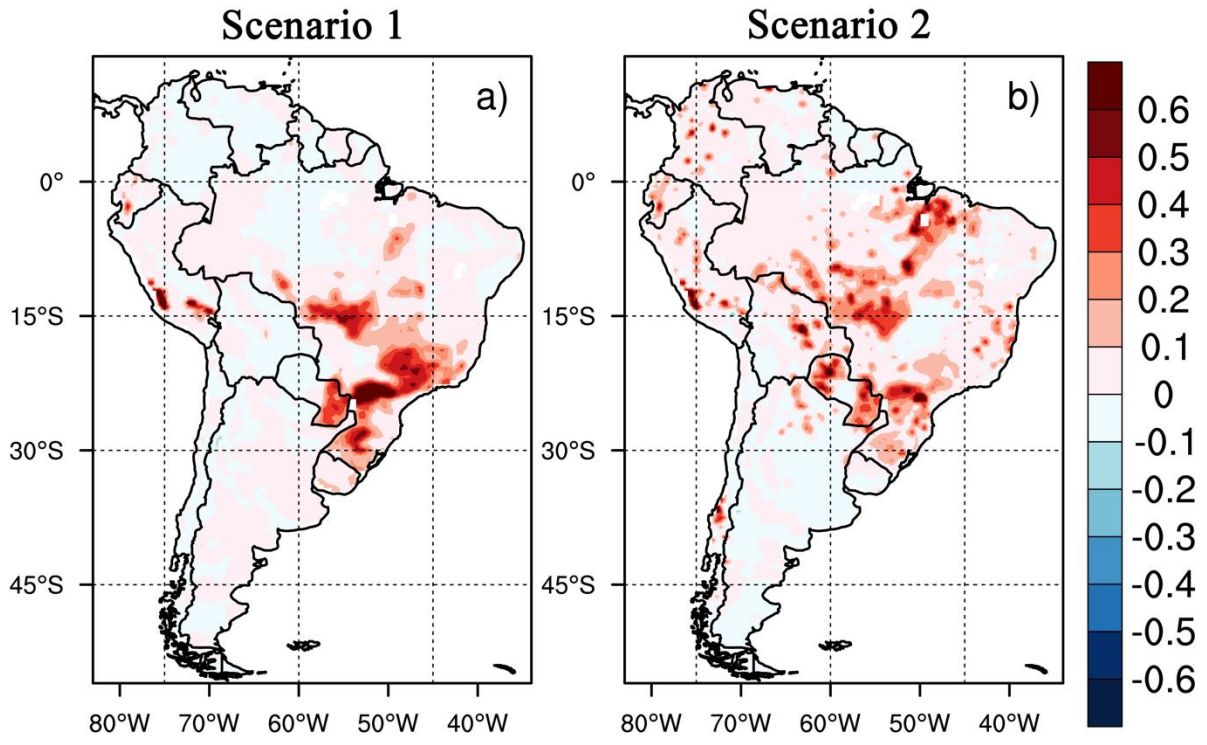
Figure S1. Changes of the annual average surface wind velocity (in m/s).
