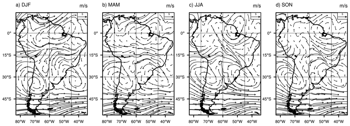
Figure S2. Seasonal atmospheric circulation at 800mb in experiment Land_1980.
