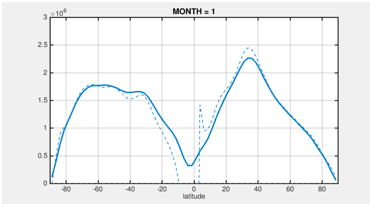
Monthly MSE diffusivity ( \cos\phi K_z ) in AQUA-AM2.1 control run computed from the optimization (solid) and the direct method (dashed).
