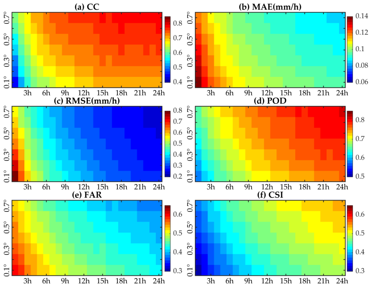
Figure S2. The distribution of grid-averaged performance metrics for IMERG-L calculated at different spatial and temporal resolutions for the entire study period.
