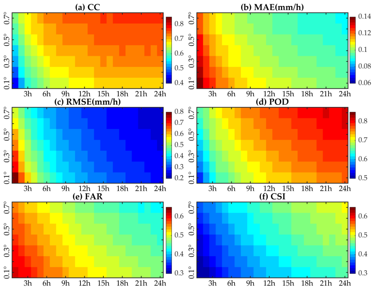
Figure S1. The distribution of grid-averaged performance metrics for IMERG-E calculated at different spatial and temporal resolutions for the entire study period.
