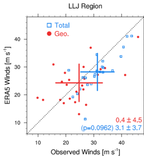
Supplemental Figure 2: The same as Fig. 7a except that the “Total” winds are not rotated here and are the true total wind speeds.
